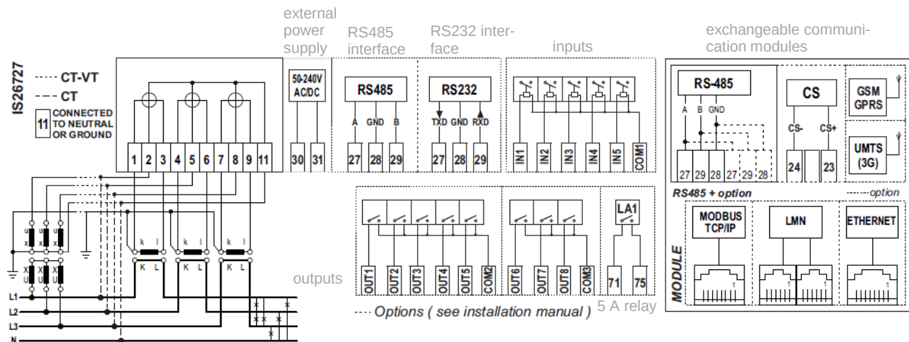
Figure 3: Meter connection diagram – CT, CT/VT connection, 3-phase 4-wire system, modular version
