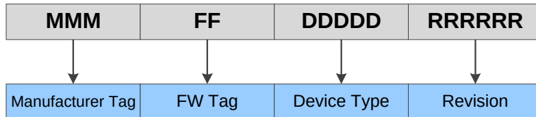
Figure 97: Firmware Identification Structure
