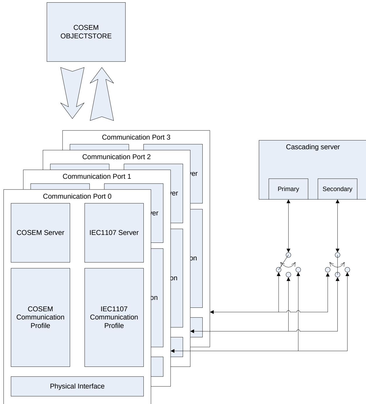
Figure 87: Meter communication model
