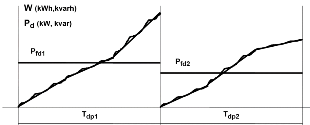
Figure 12: Demand measurement in a fixed demand period
