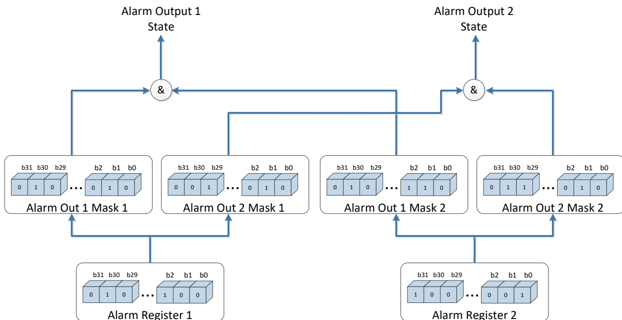
Figure 60: Alarm outputs generation
