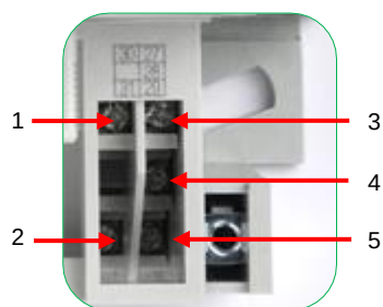
Figure 18: Additional terminals – external power supply and RS485/RS232
