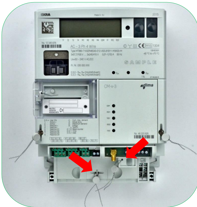
Figure 78: COP5 and a communication module seal positions
