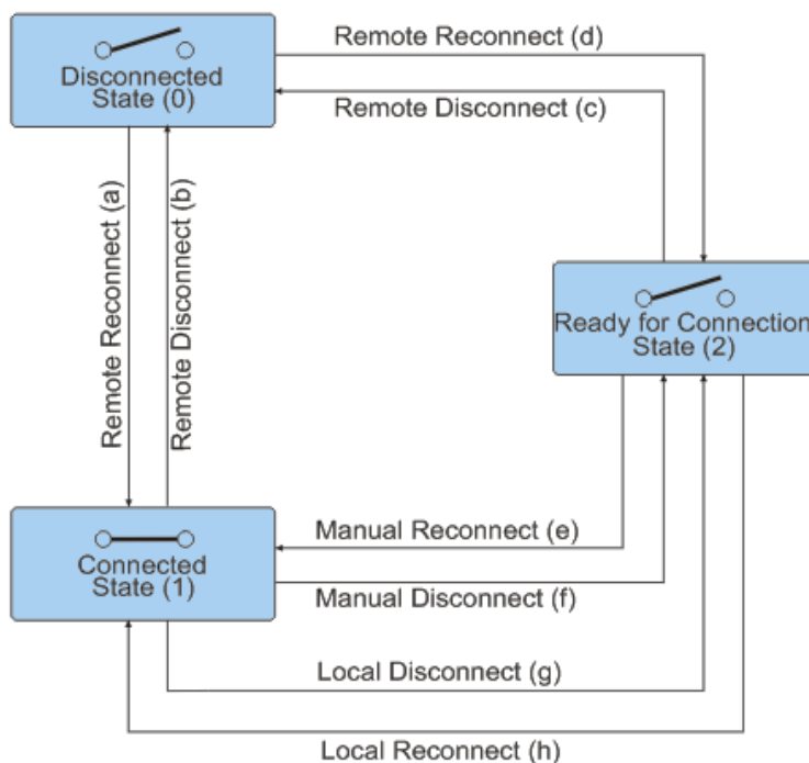
Figure 66: Operation of disconnect control object
