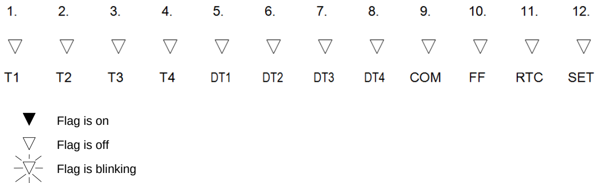
Figure 35: Display cursors legend
