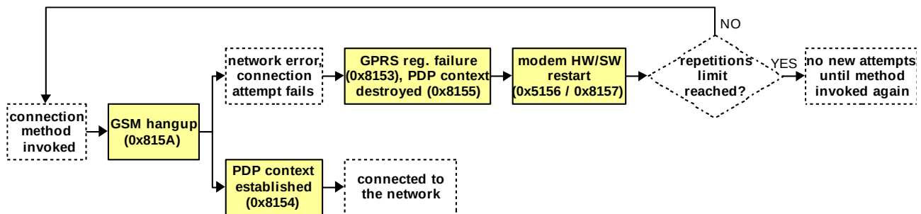
Figure 84: Auto connect operation in modes 103 and 104 when a connection method is invoked
