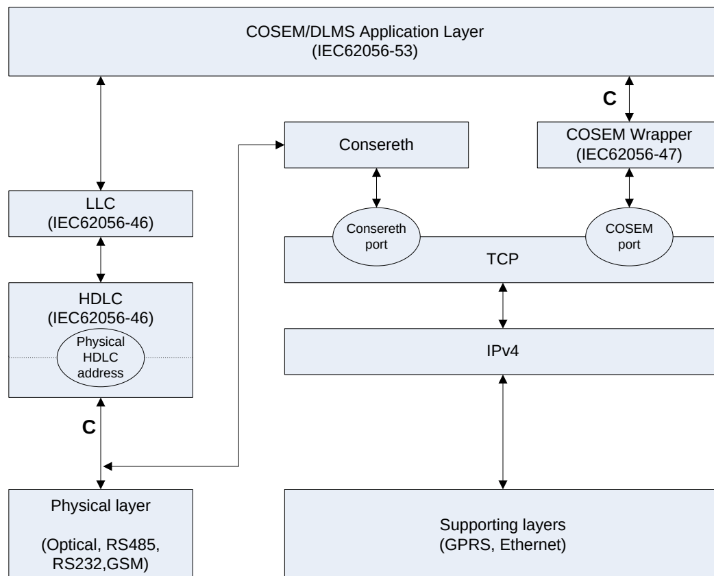
Figure 85: COSEM communication profiles
