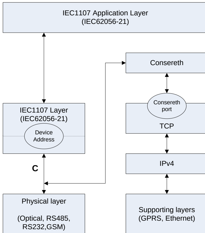
Figure 86: IEC 62056-21 (IEC 1107) communication profiles
