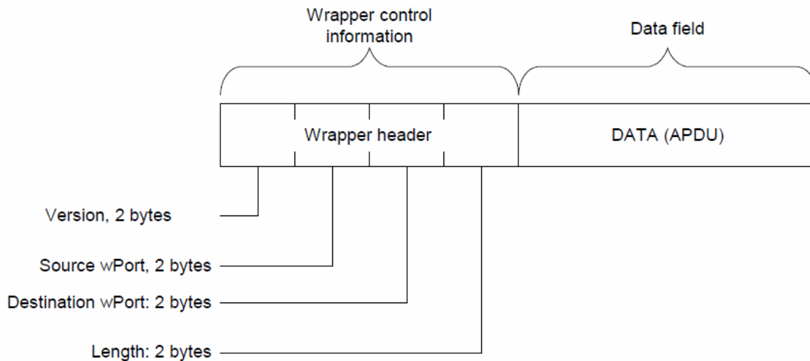
Figure 88: The COSEM wrapper protocol data unit (WPDU)
