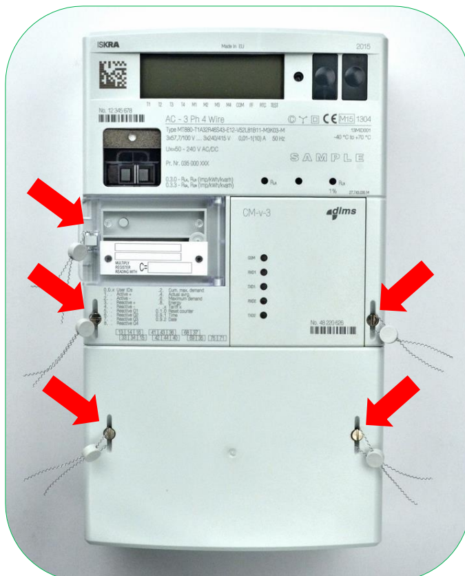
Figure 77: Meter and a terminal cover seal positions
