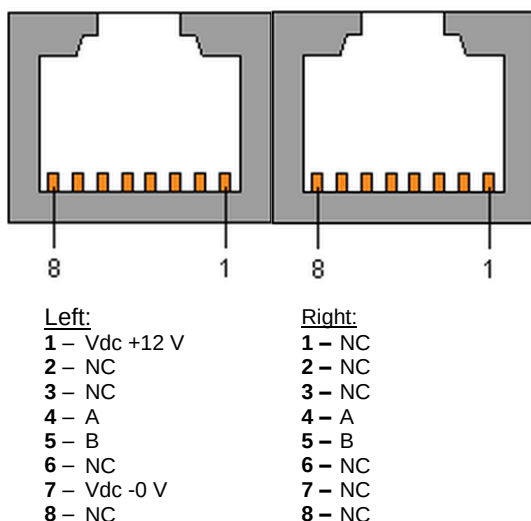
Figure 81: Description of RJ45 (8 pins) for RS485 interface connection
