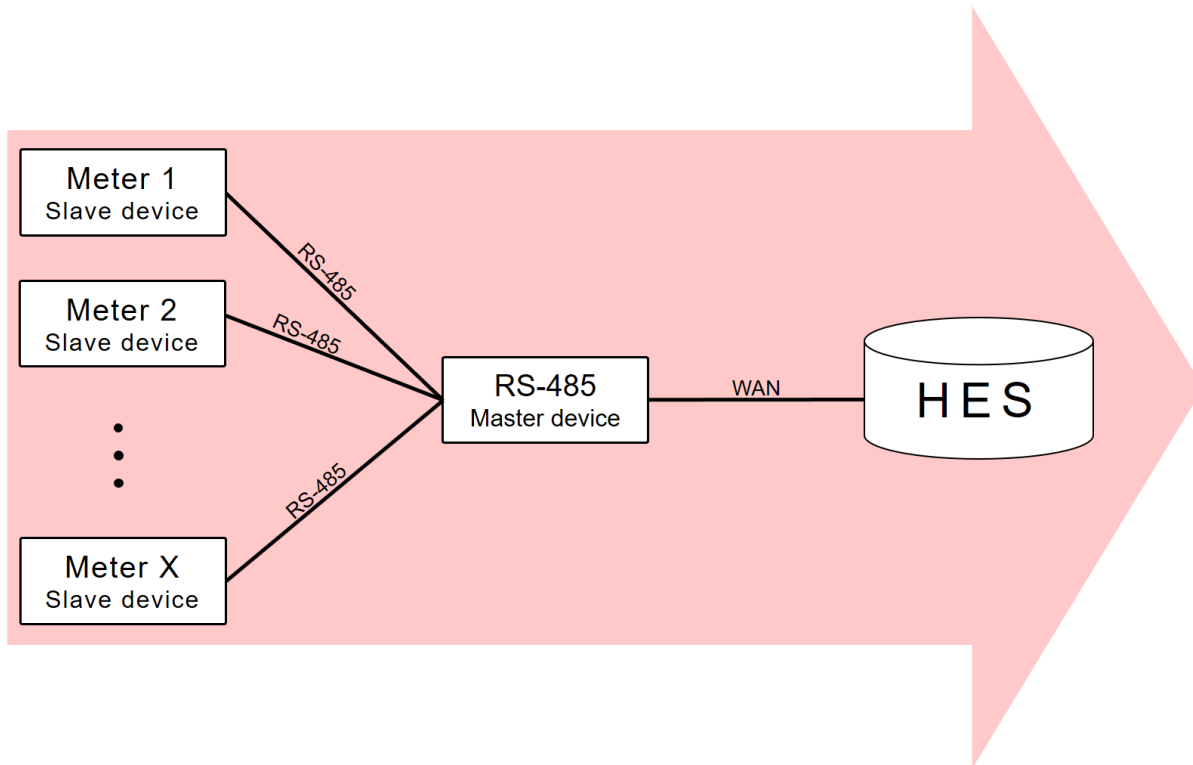
Figure 92: Flow direction of push messages over RS-485
