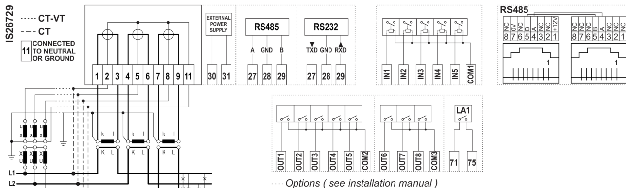
Figure 25: Example of the meter connection diagram
